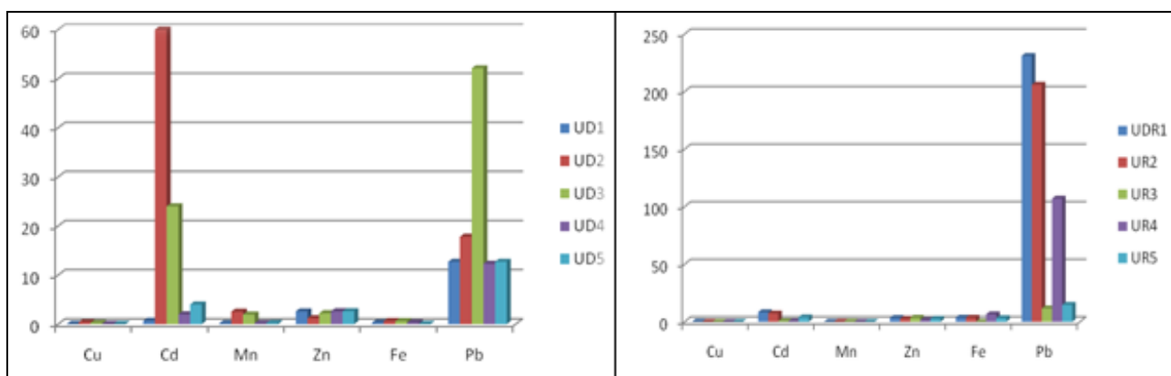
Fig 2: Contamination factor of heavy metals at different point during the dry and rainy season
